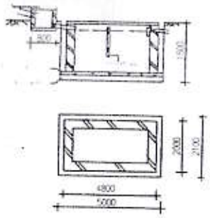
SEPTIC TANK DETAIL
