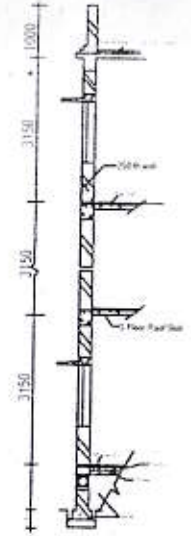
SECTIONAL ELEVATION S-S
